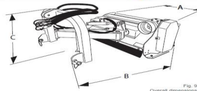
Fig. 9 Overall dimensions
